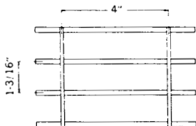
TYPE IWA (Standard Bearing)*
